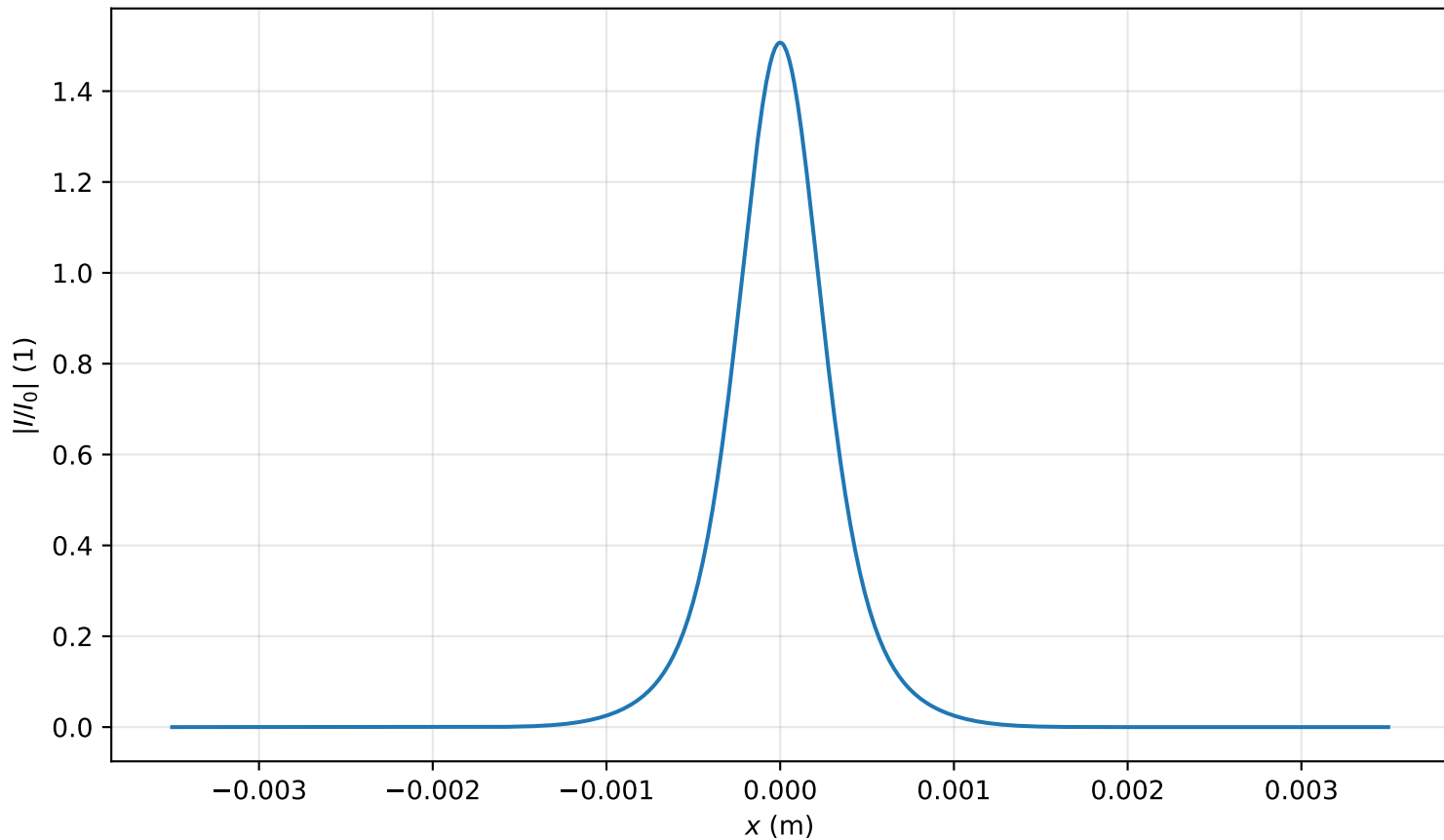
Intensity profile I(x, y = 0, z = 1.274m)/I_0 , P_{in}=0.9P_{cr} , artificial time
